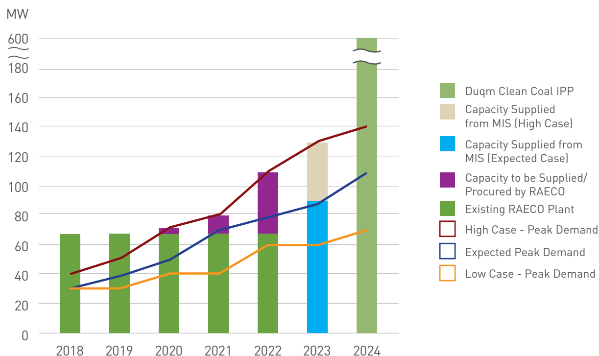
Figure 11 Resource Development Plan – Ad Duqm
