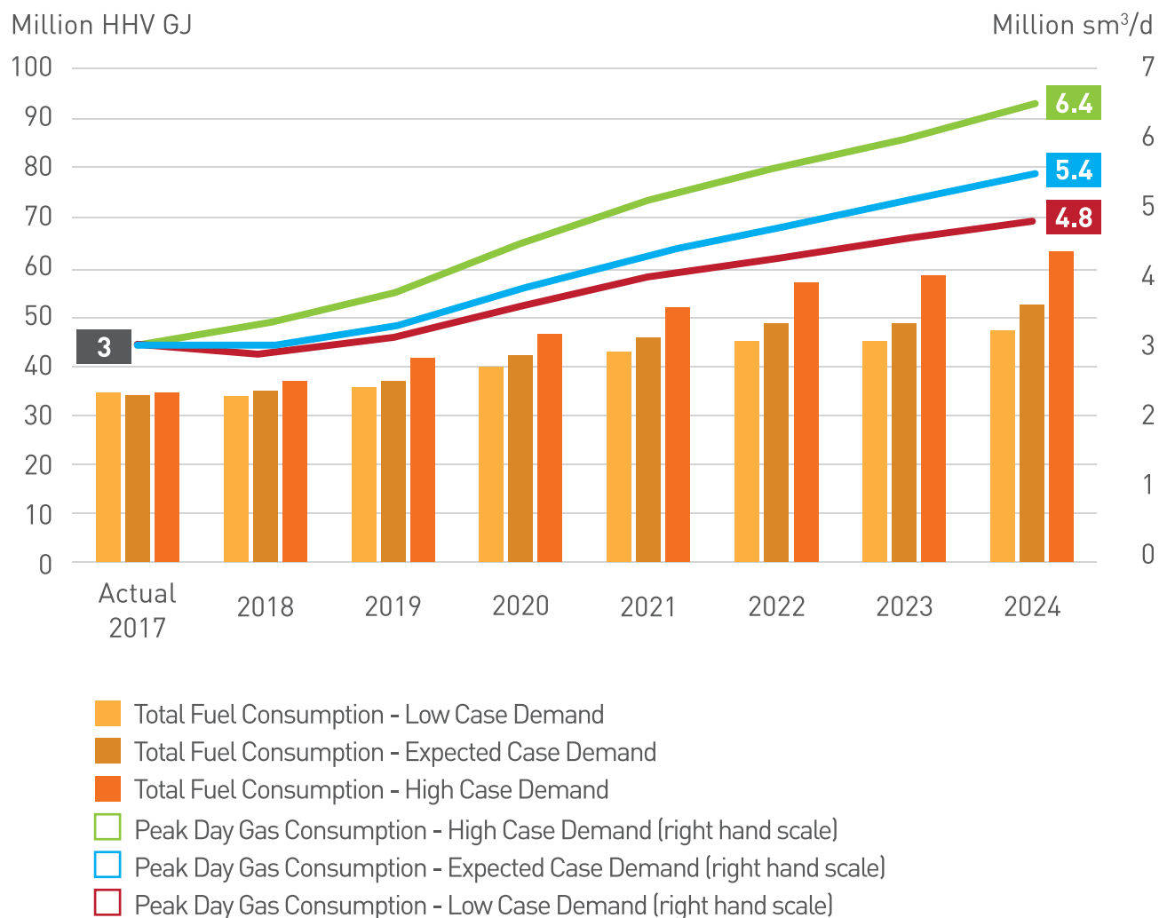
Figure 17 Projected Fuel Requirements – DPS
