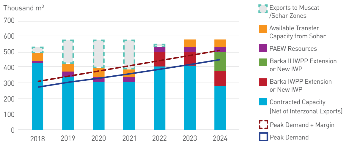
Figure 19B Resource Adequacy and Development Plan – Barka Zone
