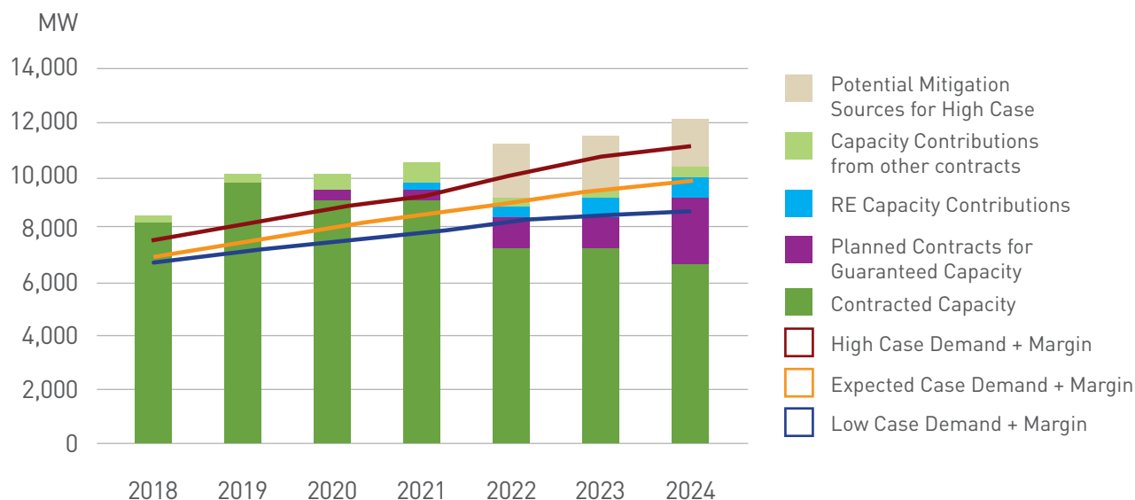
Figure 5 Resource Adequacy – MIS
