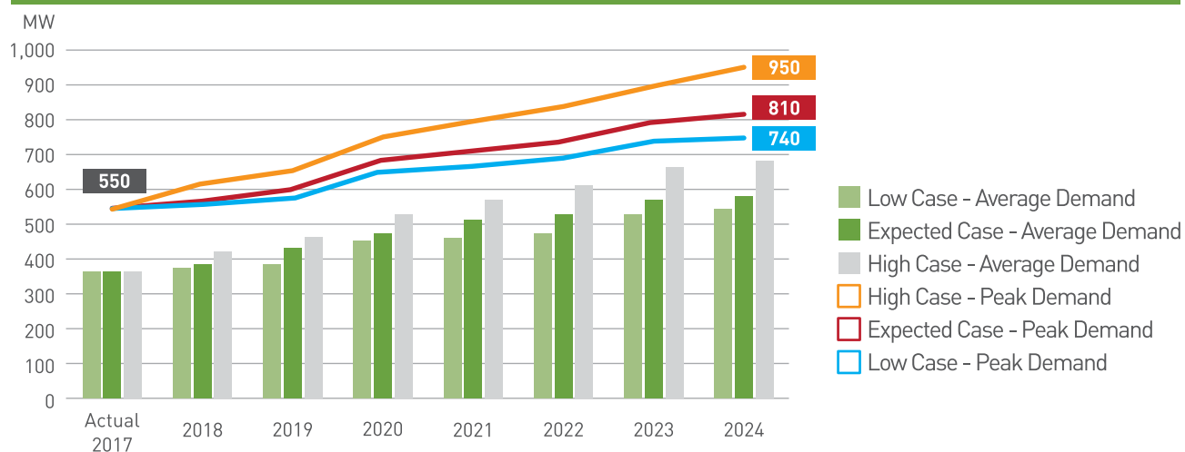
Figure 7 Electricity Demand Projections – DPS
