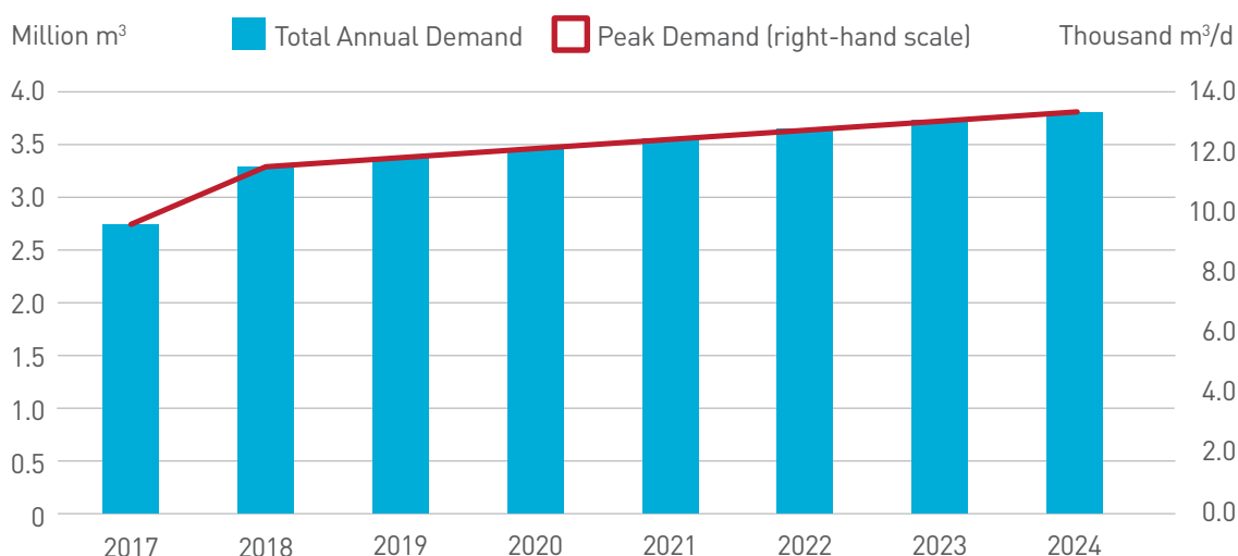
Figure 25 Peak Water Demand Projections – Musandam (Khasab City)
