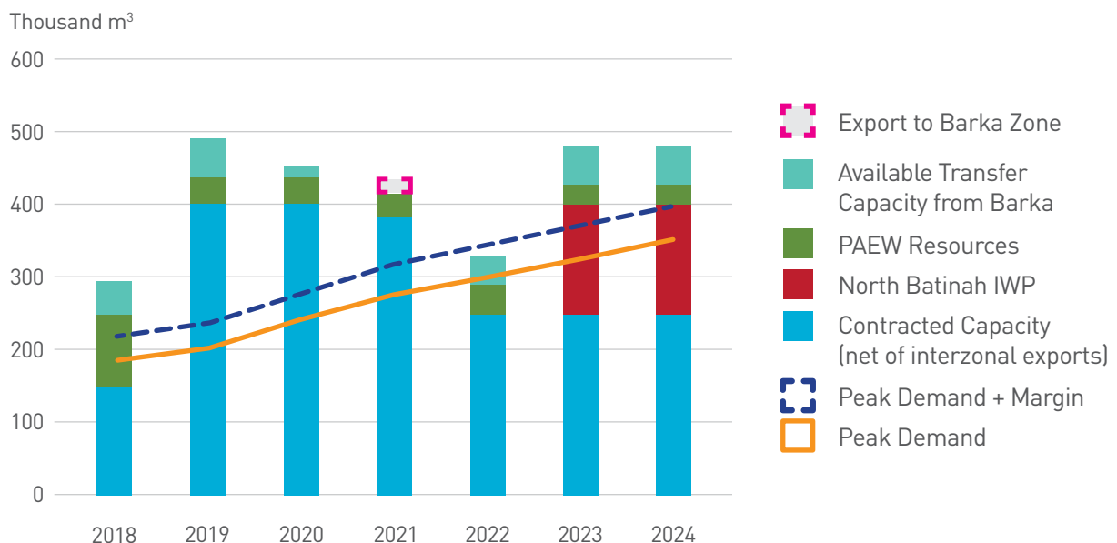
Figure 19C Resource Adequacy and Development Plan – Sohar Zone
