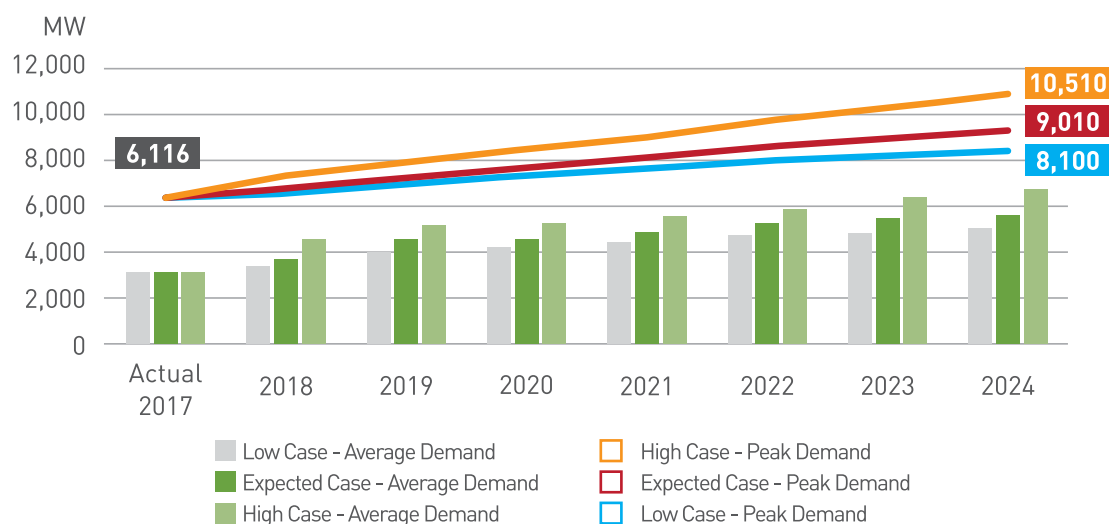
Figure 2 Electricity Demand Projections – MIS
