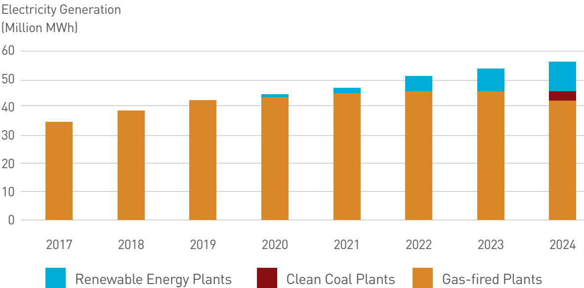
Figure 14 Fuel Shares in Electricity Generation
