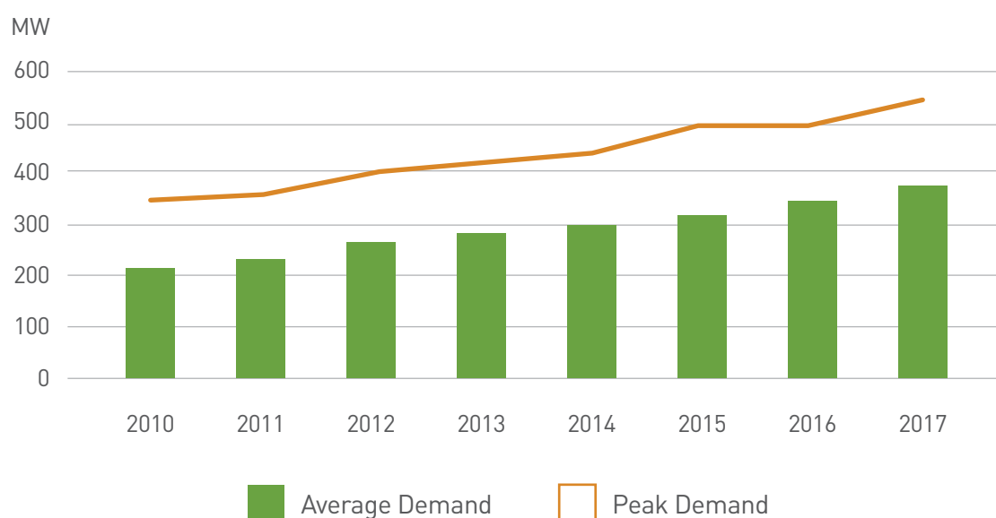
Figure 6 Historical Electricity Demand – DPS
