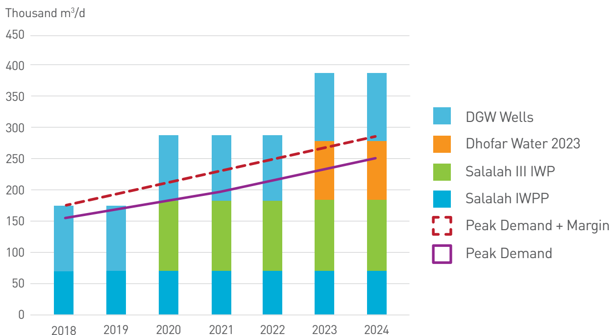
Figure 24 Resource Adequacy and Development Plan – Dhofar Cities, Jabal, and Sahal
