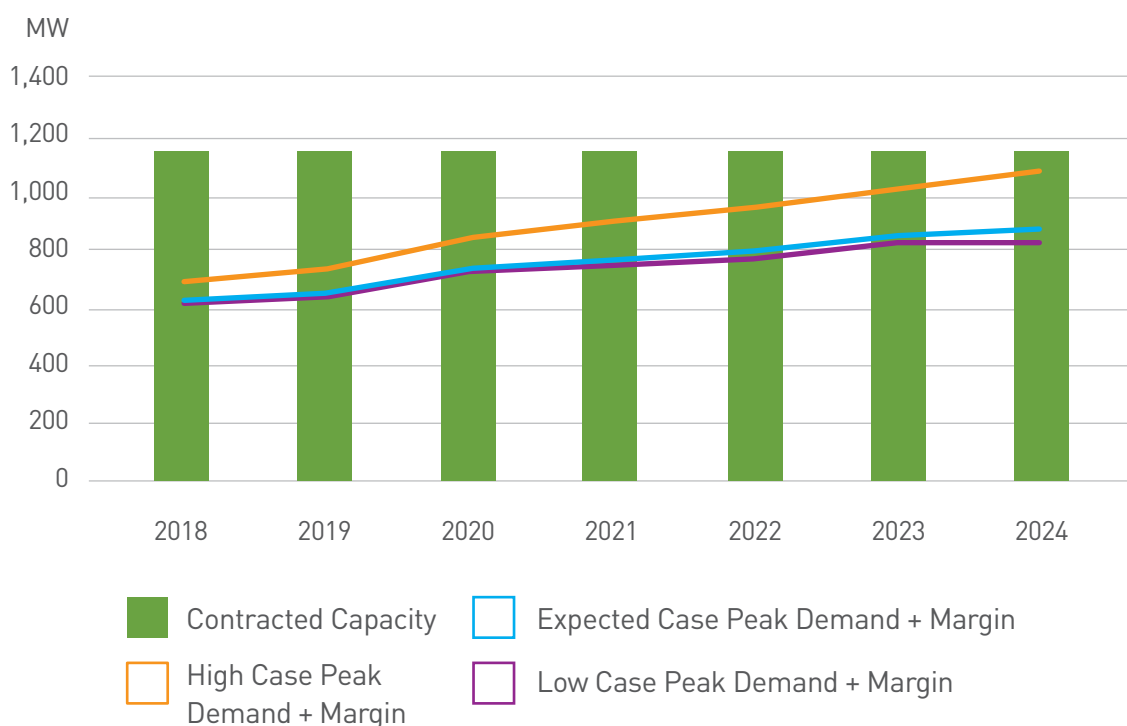
Figure 9 Resource Adequacy – DPS
