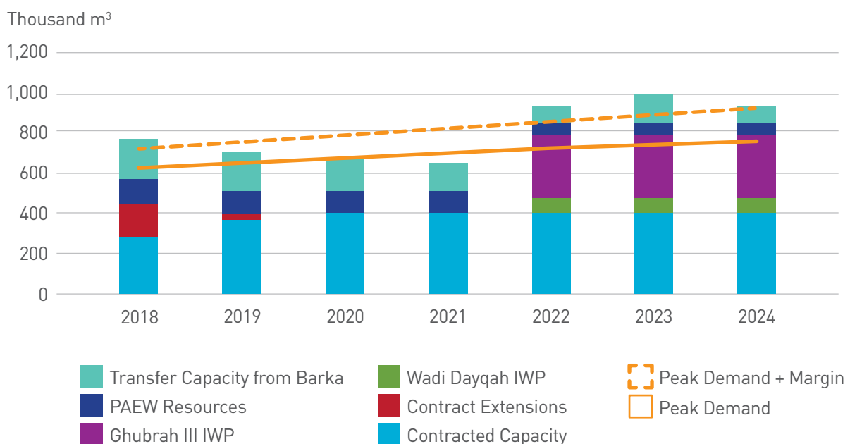
Figure 19A Resource Adequacy and Development Plan – Muscat Zone
