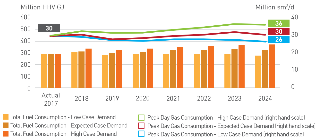
Figure 16 Projected Fuel Requirements – MIS
