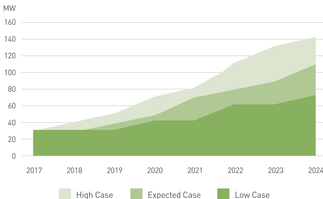
Figure 10 Electricity Demand Projections – Ad Duqm
