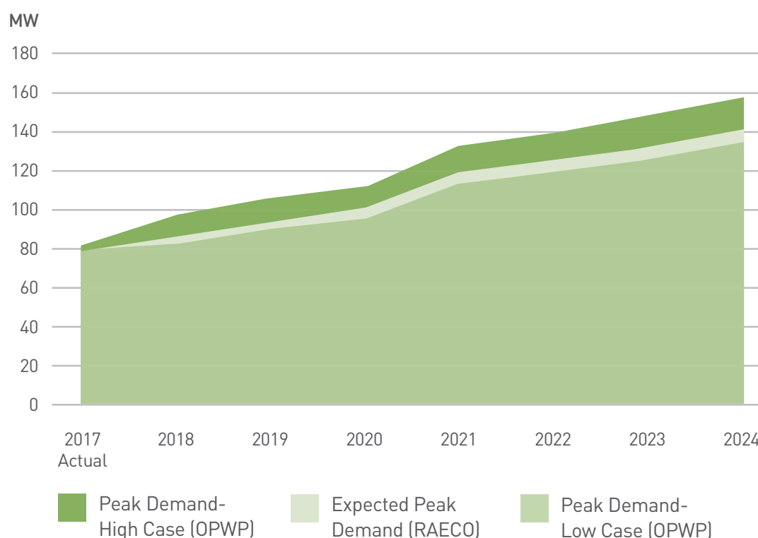
Figure 12 Electricity Demand Projections – Musandam Power System
