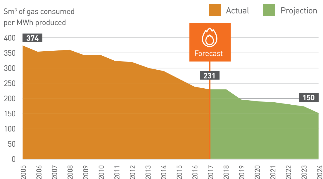
Figure 15 Gas Required per Unit of Electricity Generation – MIS
