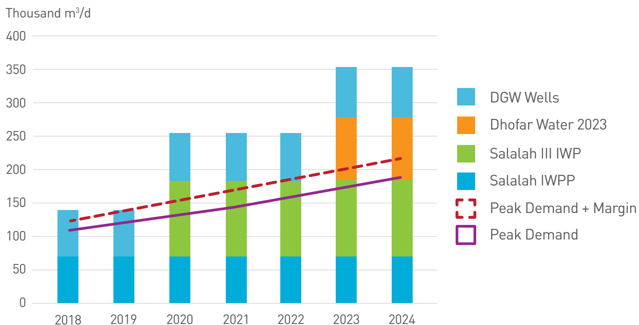
Figure 23 Resource Adequacy and Development Plan – Dhofar Cities Only
