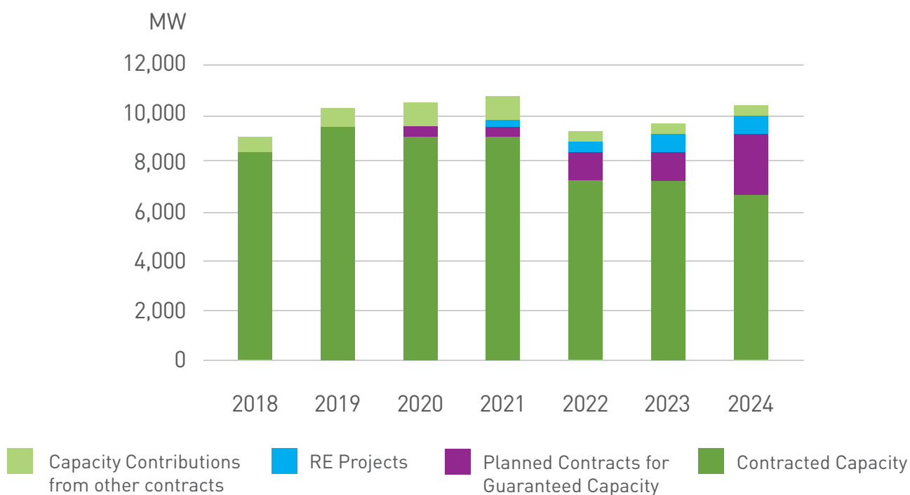
Figure 4 Capacity Contributions from Generation Resources – MIS
